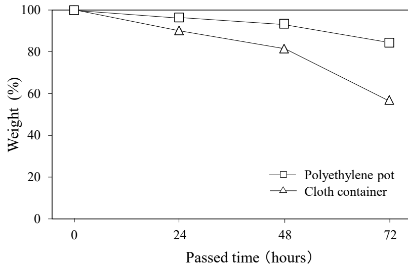
Fig. 3. Effect of container on water retention.
