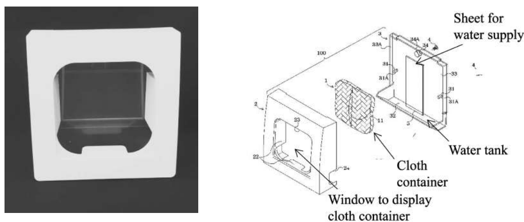
Fig. 2. Hanging frame which can be set on wall (left) and its structure (right).
