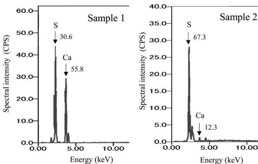
Fig. 7. X-ray fluorescence spectrum of white solid accumulated on cloth container.
